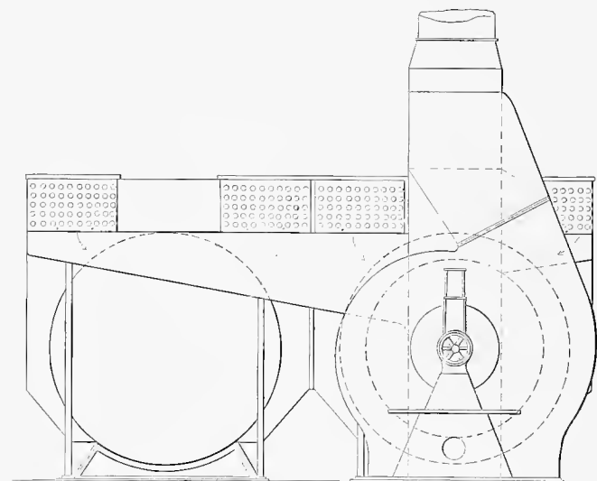
FIG. 4.—REAR ELEVATION, SHOWING POSITION OF FAN ENGINES.
